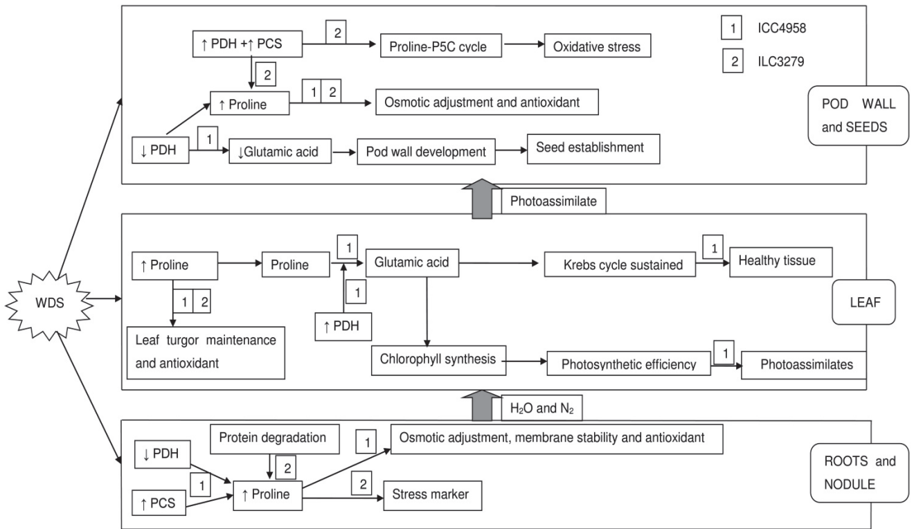
Fig. 1 Suppl. Proline metabolism in different tissues (roots, nodules, leaves, pod wall, and seeds) of chickpea cultivars (ICC4958 and ILC3279) under water deficit stress (WDS). PCS - \Delta^1 -pyrroline-carboxylate synthetase, PDH - proline dehydrogenase.
