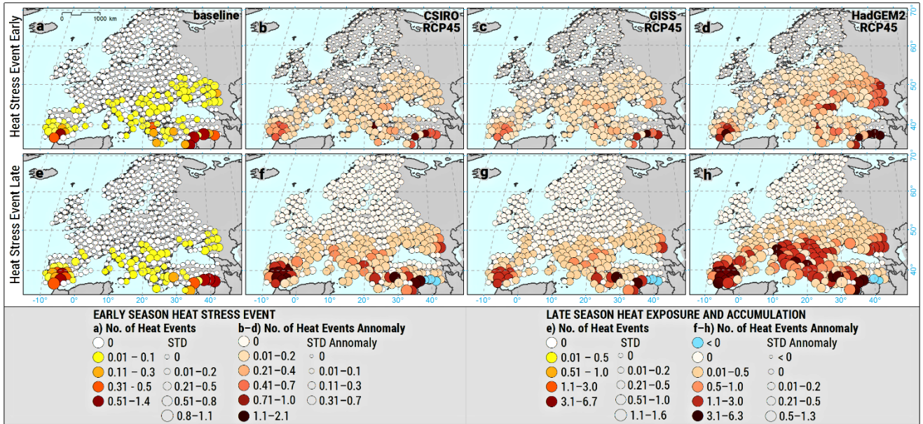
Fig. 4 Suppl. Probability of occurrence of at least 2 d with T_{max} > +31\text{ }^{\circ}\text{C} in the early season (January - May) (a) and T_{max} > +35\text{ }^{\circ}\text{C} for the period of late (June - October) season during 1981 - 2010 (e). The expected change compared to baseline is provided in the next three columns for CSIRO-RCP4.5 (b,f), GISS-RCP4.5 (c,g), and HadGEM-RCP4.5 (d,h) scenarios that represent period 2041 - 2060. The size of the circle is corresponding to the standard deviation (STD) of the given parameter over 300 individual yearly simulation. The STD of the anomaly represents increase (when \text{STD} > 1.0 ) or decrease (when \text{STD} < 1.0 ) of annual variability of the given indicator with respect to the baseline.
